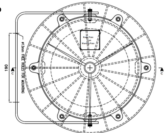
Plan View of Well Glass Fitting (TYPE - 1)
